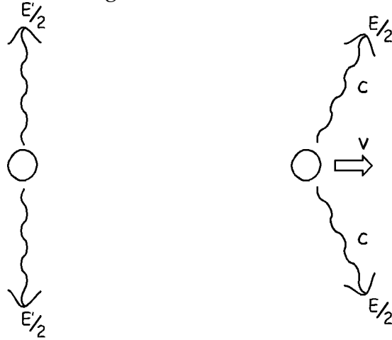
Figure 16. A mass emits two quantities of radiation
