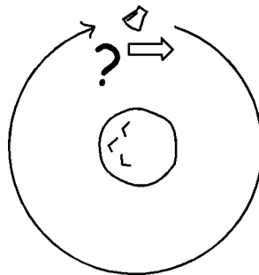
Figure 7. An easy problem in Newtonian physics.
