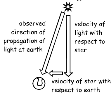
Figure 12. Stellar aberration
