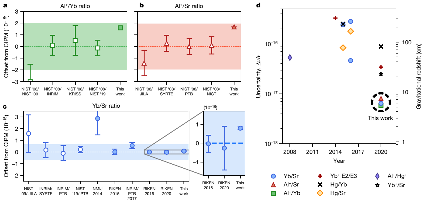
Fig. 3 | Comparison of measured frequency ratios with previous results. a–c , Values of ratios \text{Al}^+/\text{Yb} ( a ), \text{Al}^+/\text{Sr} ( b ) and \text{Yb}/\text{Sr} ( c ), reported as fractional offsets from the ratios of current CIPM recommended frequencies ( \text{Al}^+ , 1121015393207857.3 Hz; \text{Yb} , 518295836590863.6 Hz; and \text{Sr} , 429228004229873.0 Hz, with fractional uncertainties of 1.9 \times 10^{-15} , 5 \times 10^{-16} and 4 \times 10^{-16} , respectively) 15 . The shaded region in each plot indicates the standard uncertainty of the CIPM ratio, determined from the quadrature sum of the absolute frequency uncertainties. Ratios based on absolute frequency measurements are presented with open symbols, whereas frequency ratios based only on optical clock measurements are presented with filled symbols. For \text{Yb}/\text{Sr} ( c ), a subset of the most accurate absolute frequency measurements is displayed 44–49 in addition to all direct optical frequency ratios 4,21,28,50 , and an
