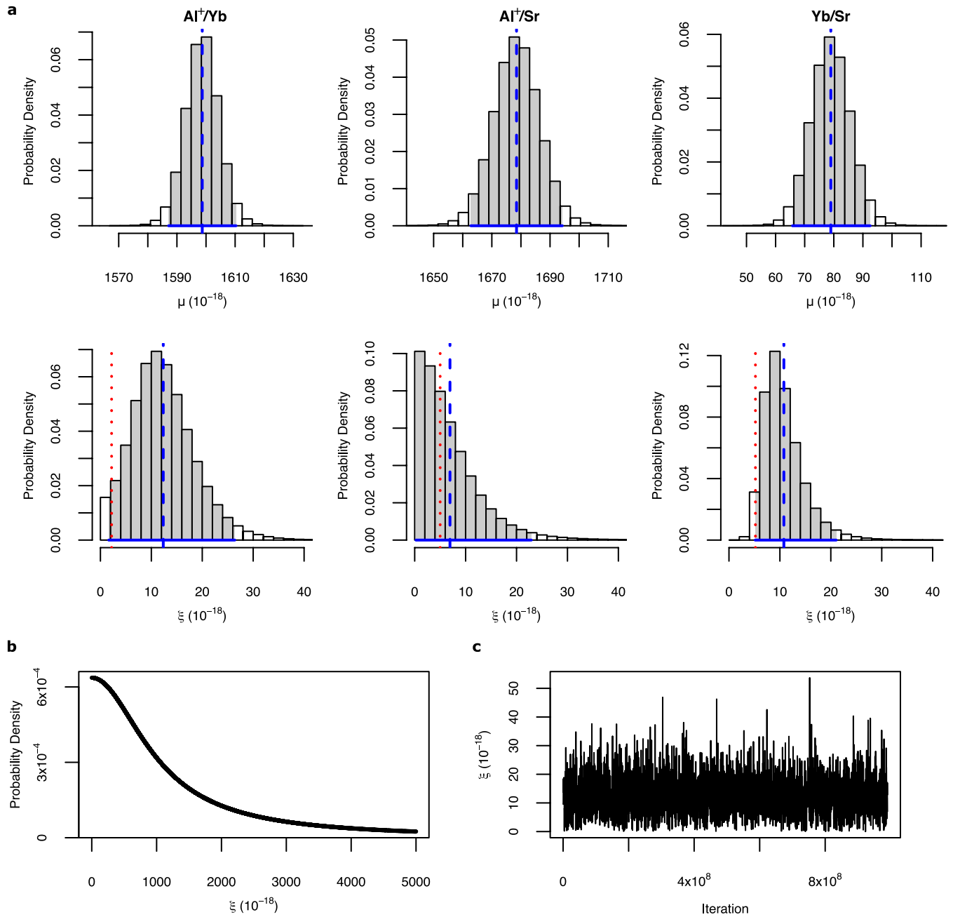
Extended Data Fig. 3 | Results of the Bayesian analysis. a, Posterior distributions for the ratio values \mu (top row) expressed here as a fractional offset from the current recommended CIPM values 15 , and for the between-day variability \xi (bottom row). Left column, ratio \text{Al}^+/\text{Yb} ; middle column, ratio \text{Al}^+/\text{Sr} ; right column, ratio \text{Yb}/\text{Sr} . The blue dashed lines denote our estimate for these parameters, the posterior mean. The shaded areas and blue lines on the bottom of each plot denote the 95% credible intervals and the red dotted lines denote the static uncertainties due to systematic effects. The posterior
