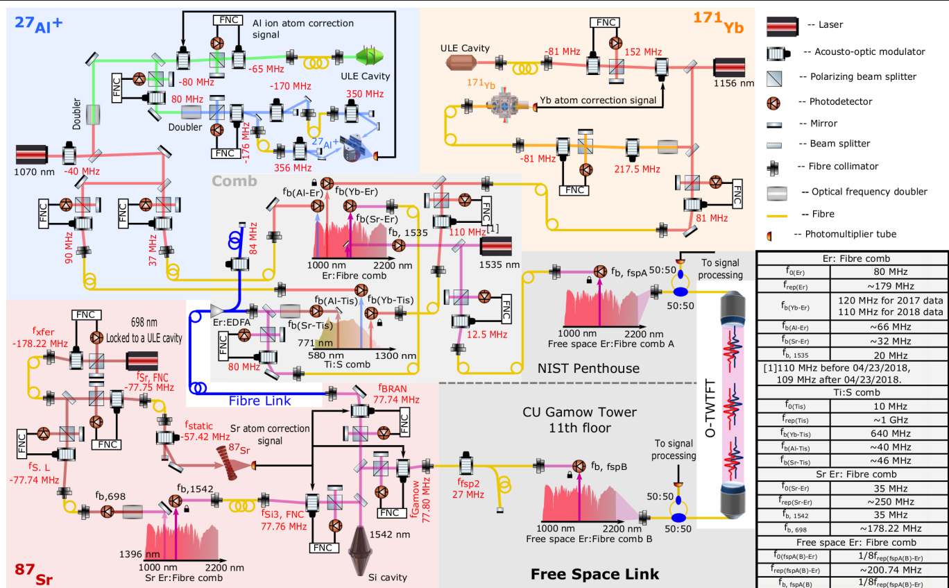
Extended Data Fig. 1 | Diagram of the Boulder Atomic Clock Optical Network (BACON). The Al + ion optical clock (blue shaded area), the Yb optical lattice clock (orange shaded area), the Er:fibre comb (light grey shaded area) and the Ti:S comb (light grey shaded area) are located in Building 81 of NIST. The Sr optical lattice clock (pink shaded area) is located in the basement of JILA. The free space link (grey shaded area) includes two parts (split by the dashed line): one part is located in the NIST Building 1 penthouse and another part is located at the 11th floor of the Gamow tower at the University of Colorado. The Er:fibre comb and the Ti:S comb at NIST are locked to the Yb optical clock. The Er:fibre comb in the Sr optical clock lab is locked to the Si cavity and is used to
