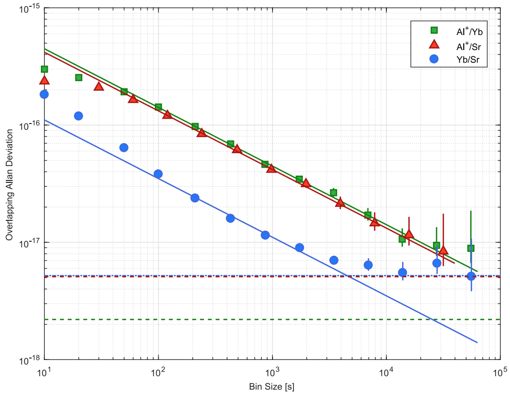
Extended Data Fig. 2 | Long-term stability of concatenated ratio data as characterized by the overlapping Allan deviation. The data plotted include all measurements that were taken at the nominal operating conditions over the course of the measurement campaign with total measurement durations as follows: 165,240 s, 94,760 s and 167,140 s for \text{Al}^+/\text{Yb} , \text{Al}^+/\text{Sr} and \text{Yb}/\text{Sr} , respectively. For the \text{Al}^+/\text{Yb} ratio, in addition to the data that contributed to the final ratio, we include two extra days of data (27 February 2018 and 2 March 2018) that were used in the evaluation of the \text{Al}^+ second-order Zeeman shift as described in ref. 6 . Although acquired in very similar experimental conditions, these datasets are excluded from frequency ratio estimate to avoid statistical
